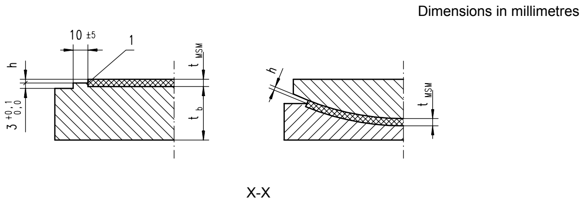
Figure B.1 — Details of MSM ® recess and relief
