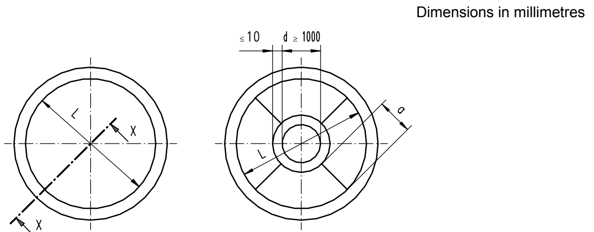
Figure B.3 - Subdivision of recessed MSM ® sheets for spherical sliding surfaces
